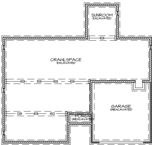
1 FOUNDATION PLAN A-3
